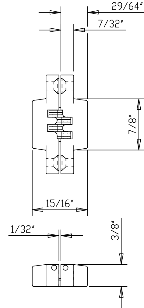
HINGE CLOSED TOP VIEW CUT AWAY
