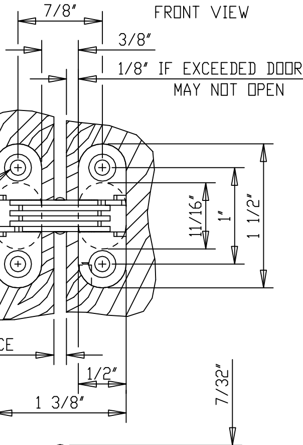
HINGE CLOSED FRONT VIEW CUT AWAY
