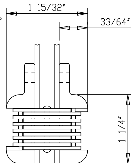
HINGE OPEN 180° FRONT VIEW
