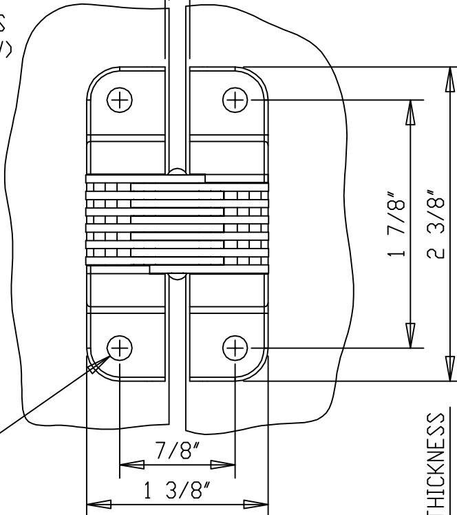
HINGE CLOSED FRONT VIEW
