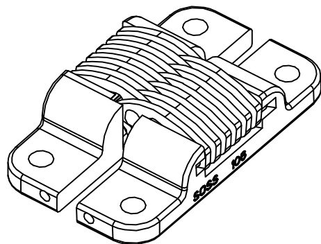
HINGE CLOSED ISOMETRIC VIEW
