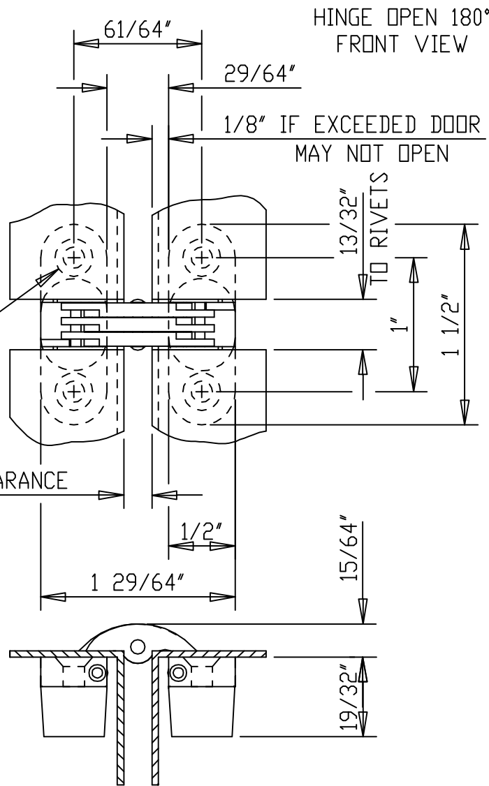
HINGE OPEN 180° TOP VIEW
