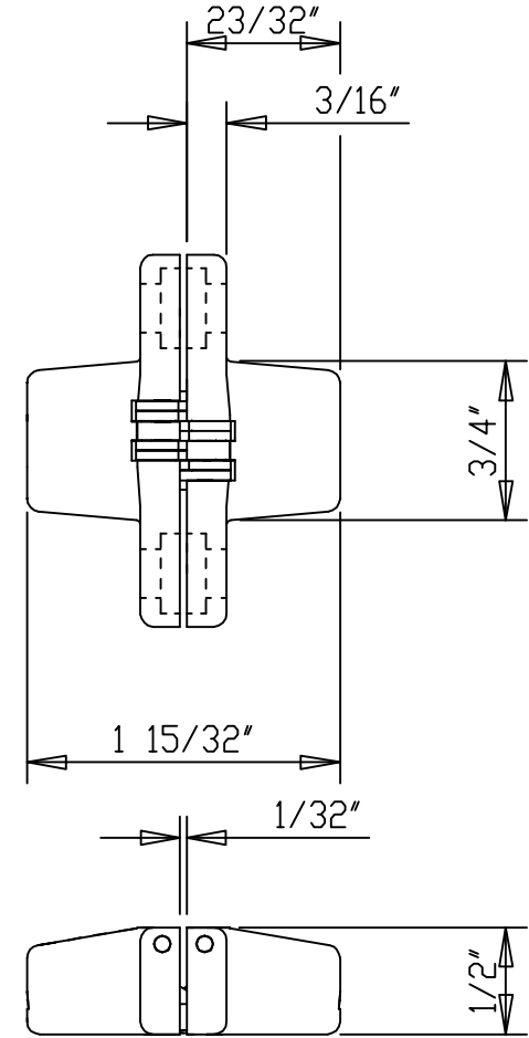
HINGE CLOSED FRONT VIEW CUT AWAY
