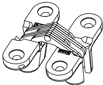
HINGE OPEN 180° ISOMETRIC VIEW
