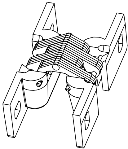
HINGE OPEN 180° ISOMETRIC VIEW
