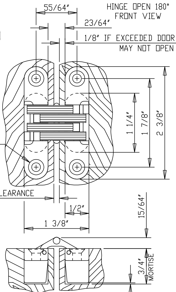
HINGE OPEN 180° TOP VIEW CUT AWAY
