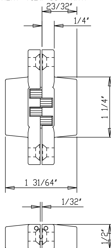
HINGE CLOSED FRONT VIEW CUT AWAY
