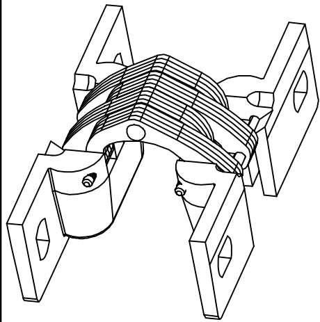
HINGE OPEN 180° ISOMETRIC VIEW
