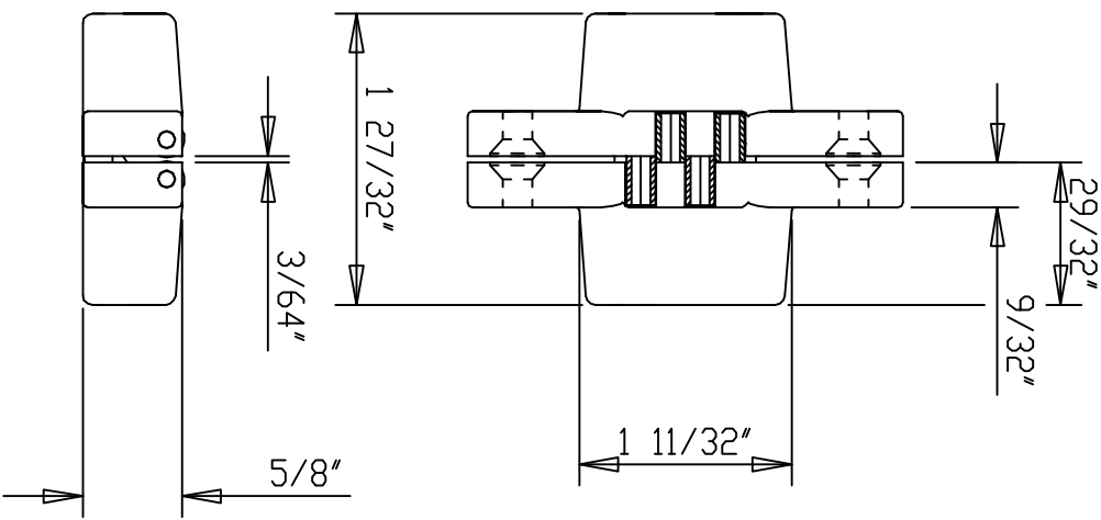
HINGE CLOSED TOP VIEW CUT AWAY
