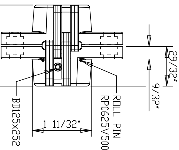
HINGE CLOSED FRONT VIEW CUT AWAY
