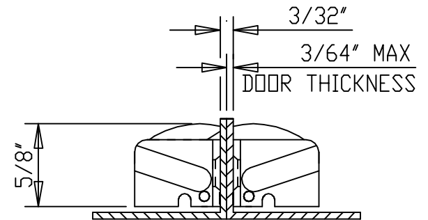
HINGE CLOSED° TOP VIEW
