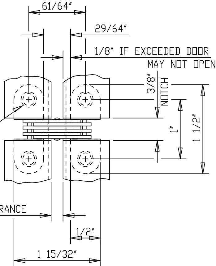
HINGE OPEN 180° FRONT VIEW
