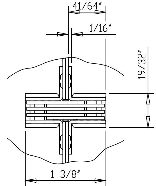
HINGE CLOSED FRONT VIEW
