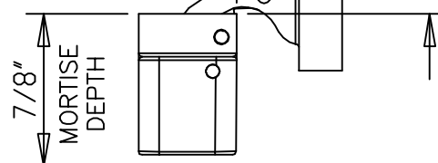
HINGE OPEN 90° TOP VIEW CUT AWAY
