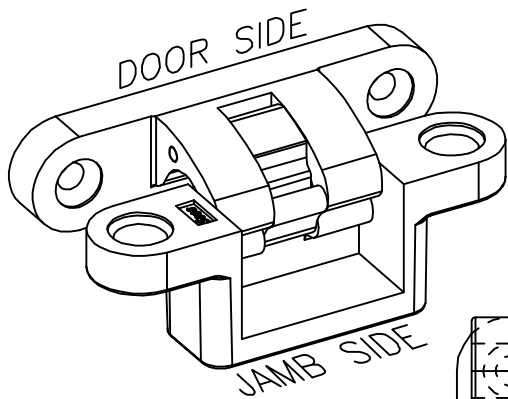
HINGE OPEN 90° ISOMETRIC VIEW
