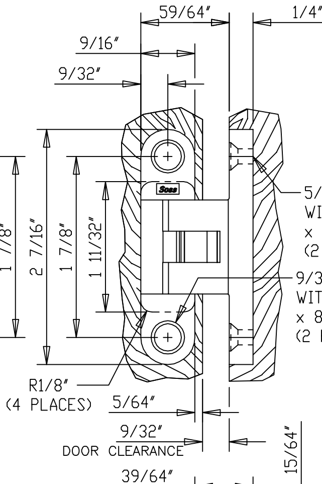
HINGE OPEN 90° VIEW
