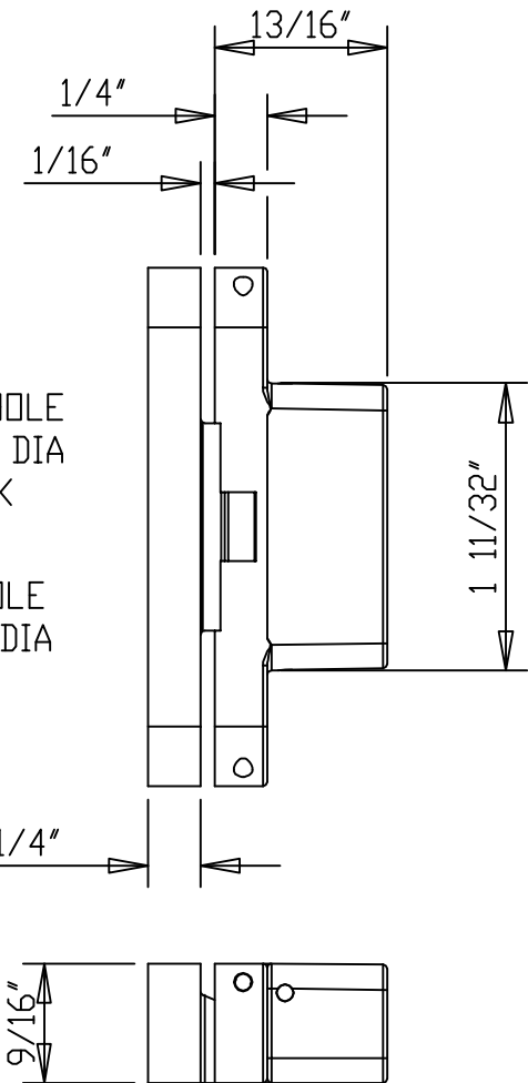
HINGE CLOSED FRONT VIEW CUT AWAY
