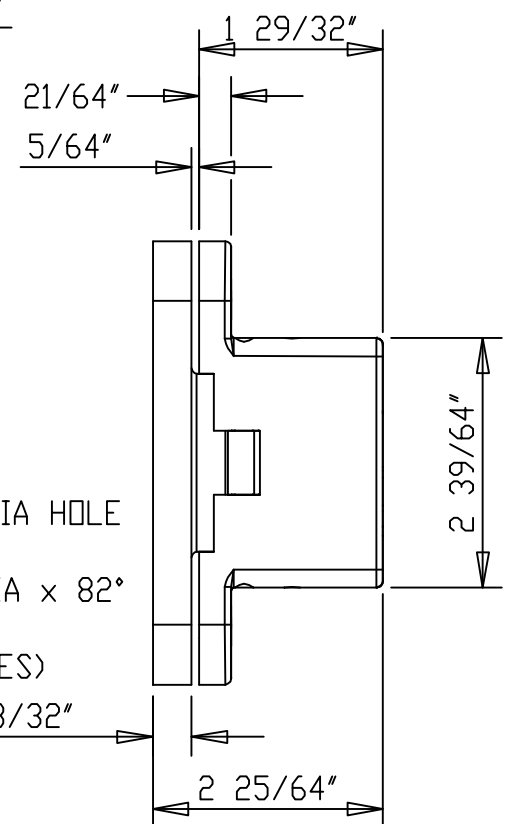
HINGE CLOSED FRONT VIEW CUT AWAY
