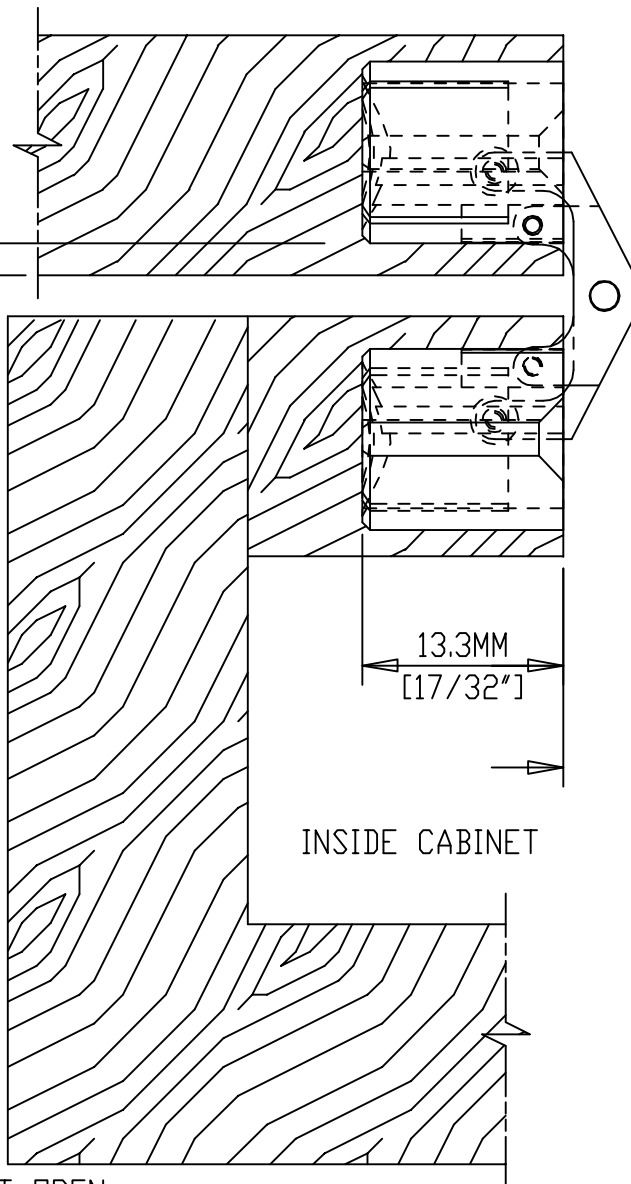
HINGE OPEN 180° SIDE VIEW CUT AWAY
