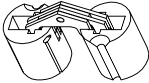
HINGE OPEN 180° ISOMETRIC VIEW
