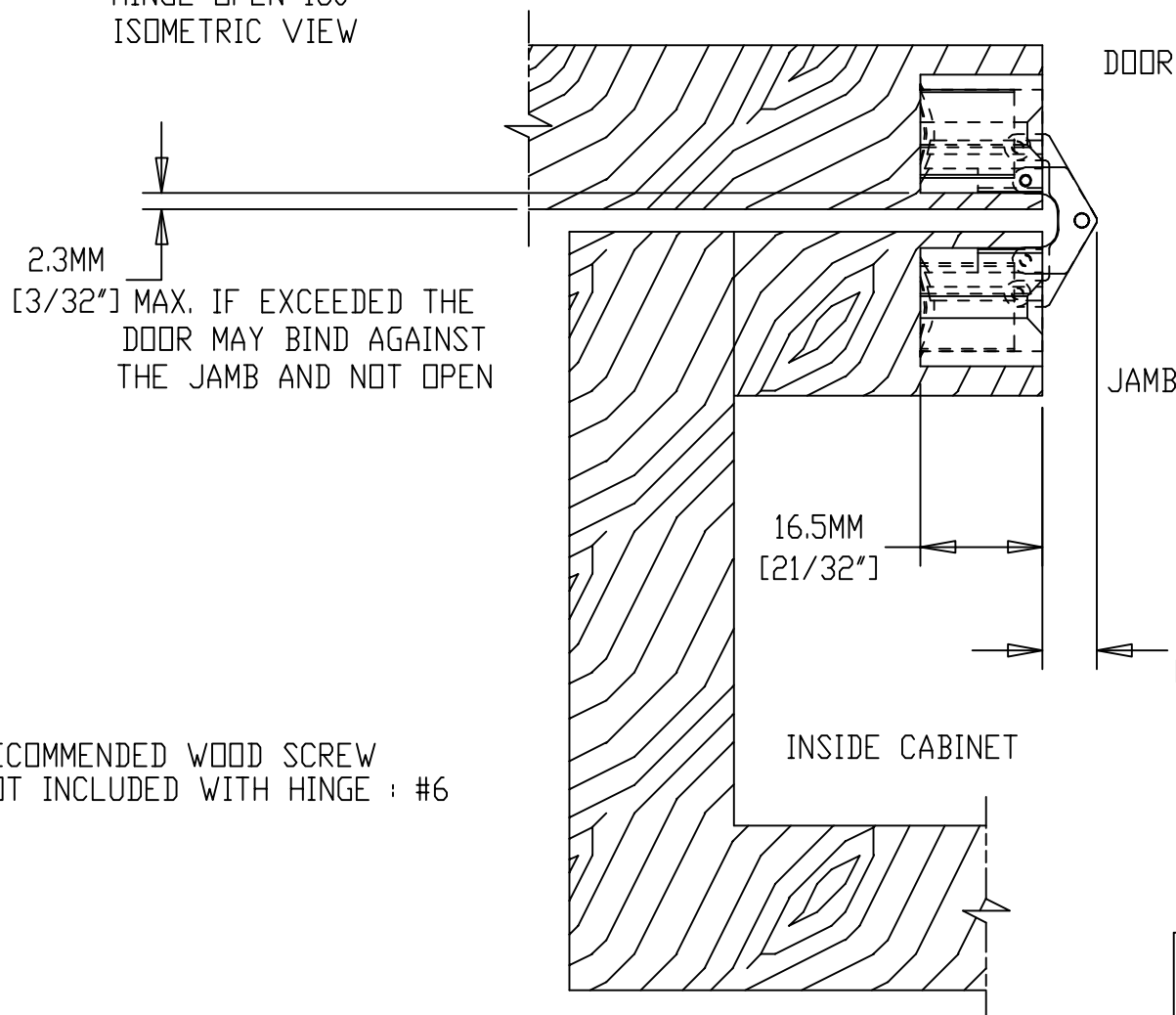
HINGE OPEN 180° SIDE VIEW CUT AWAY
