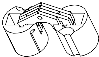
HINGE OPEN 180° ISOMETRIC VIEW
