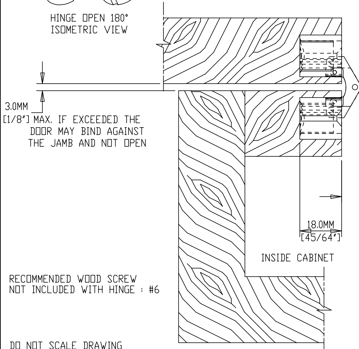
HINGE OPEN 180° SIDE VIEW CUT AWAY
