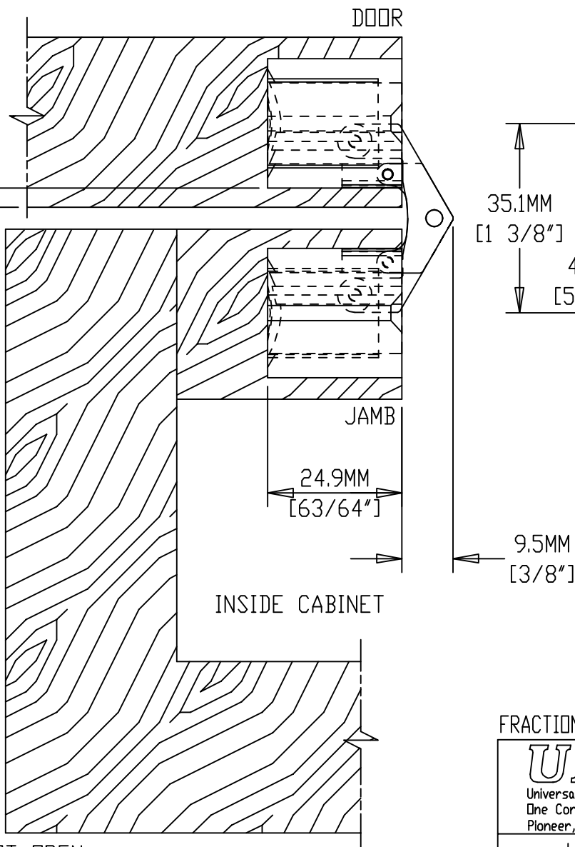
HINGE OPEN 180° SIDE VIEW CUT AWAY
