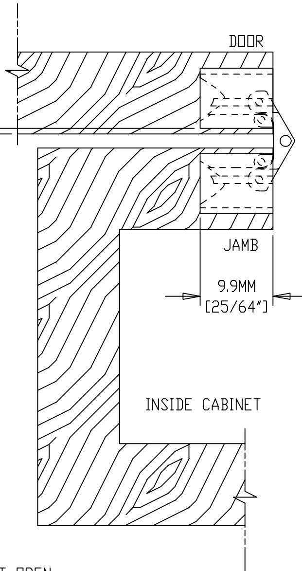
HINGE OPEN 180° SIDE VIEW CUT AWAY
