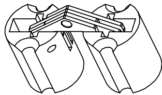
HINGE OPEN 180° ISOMETRIC VIEW
