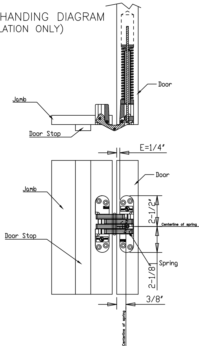
LEFT HAND & RIGHT HAND REVERSE
