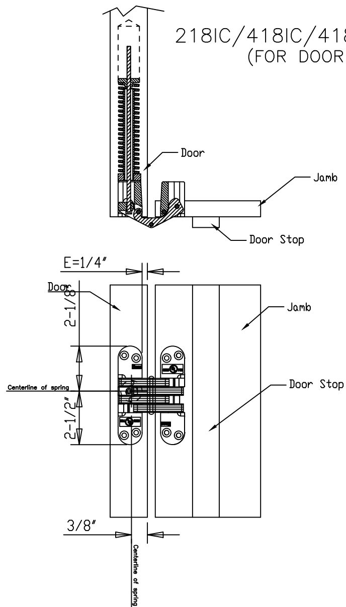
RIGHT HAND & LEFT HAND REVERSE
